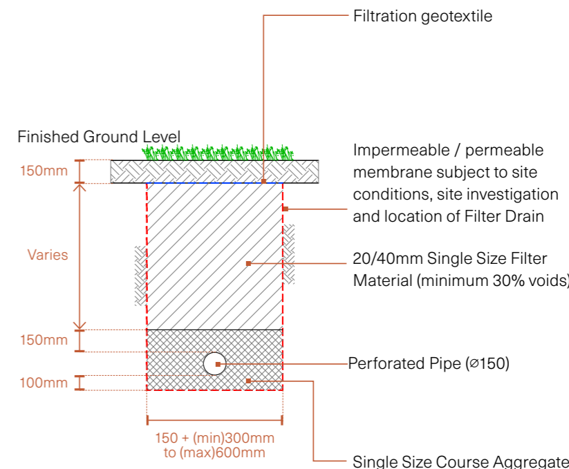
Figure 7: Typical Grassed Filter Drain Detail
