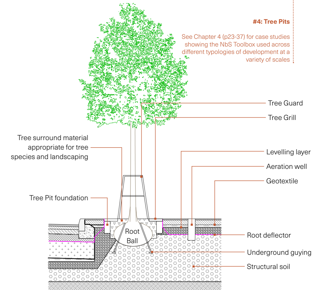
Figure 12: Tree Pit - Altrincham, Manchester
